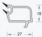
Glazing Bead (20mm) Code- DP50-EG-560
