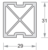
Reinforcement Code- DPDR3129
