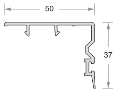
Sliding Window Interlock Code- DP67-ET-709
