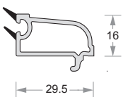
Glazing Bead (18mm) Code- DP67-ET-714
