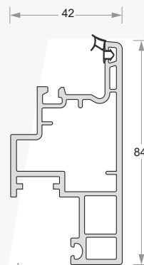
Casement Twin Villa Mesh Sash Code- DP67-ET-776
