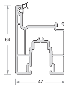
Sliding Window Sash Code- DP67-ET-706
