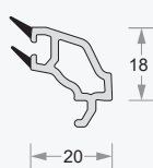
Glazing Bead (20mm) Code- DP60-EL-614
