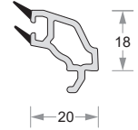
Glazing Bead (5mm) Code- DP60-EL-614
