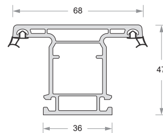
Sliding Sash Mullion Code- DP67-ET-713
