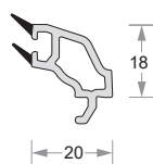
Glazing Bead (5mm) Code- DP60-EL-614
